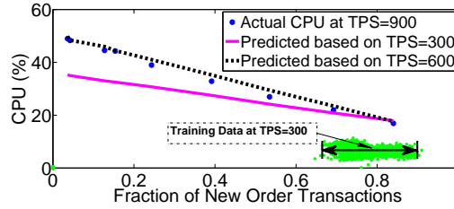
Figure 8: Predicting CPU, when varying both mixture and TPS.
